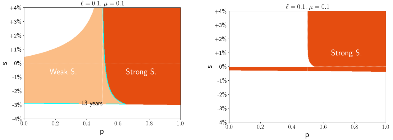
(a) \langle E_0 \rangle = \$15,000 ; \langle M_0 \rangle = \$150,000 .
